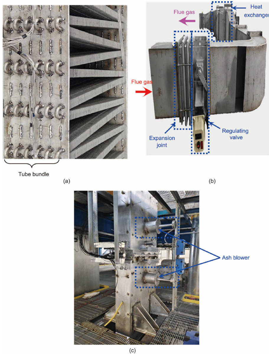
Fig. 4. Photos of the experimental setup. (a) The MSHE prototype; (b) the assembly of the flue gas-driven HSS; (c) the vertically positioned flue gas-driven HSS.
