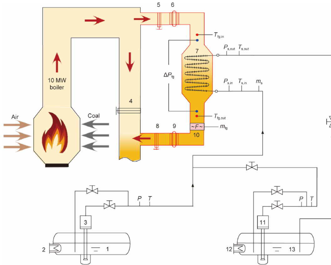
Fig. 5. Experimental setup for the flue gas-driven HSS. 1: cold salt tank; 2 and 12: electric heaters; 3: cold salt pump; 4, 5, and 8: flue gas valves; 6 and 9: expansion joints; 7: MSHE; 10: flue gas flowmeter; 11: hot salt pump; 13: hot salt tank.
