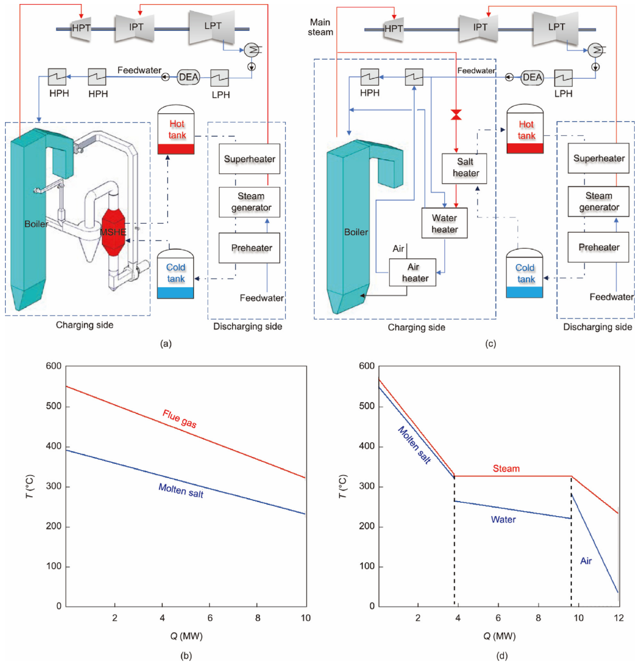
Fig. 13. Comparison of the flue gas extraction technology with the vapor extraction technology. (a) Flow chart of the flue gas-driven heat storage system; (b) T - Q curve of the flue gas-driven heat transfer; (c) flow chart of the vapor driven heat storage system; (d) T - Q curve of the vapor driven heat transfer. HPH: high pressure heater; LPH: low pressure heater; DEA: deaerator; HPT: high pressure turbine; IPT: intermediate pressure turbine; LPT: low pressure turbine.
