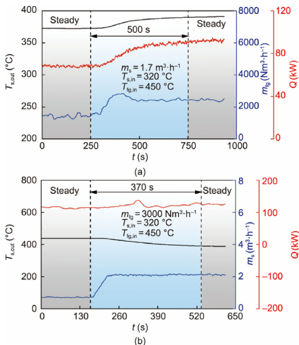
Fig. 11. Transient switch between two steady operating conditions. (a) Transient curves for m_s = 1.7\text{ m}^3\cdot\text{h}^{-1} , T_{s,in} = 320\text{ °C} , and T_{fg,in} = 450\text{ °C} ; (b) transient curves for m_{fg} = 3000\text{ Nm}^3\cdot\text{h}^{-1} , T_{s,in} = 320\text{ °C} , and T_{fg,in} = 450\text{ °C} .
