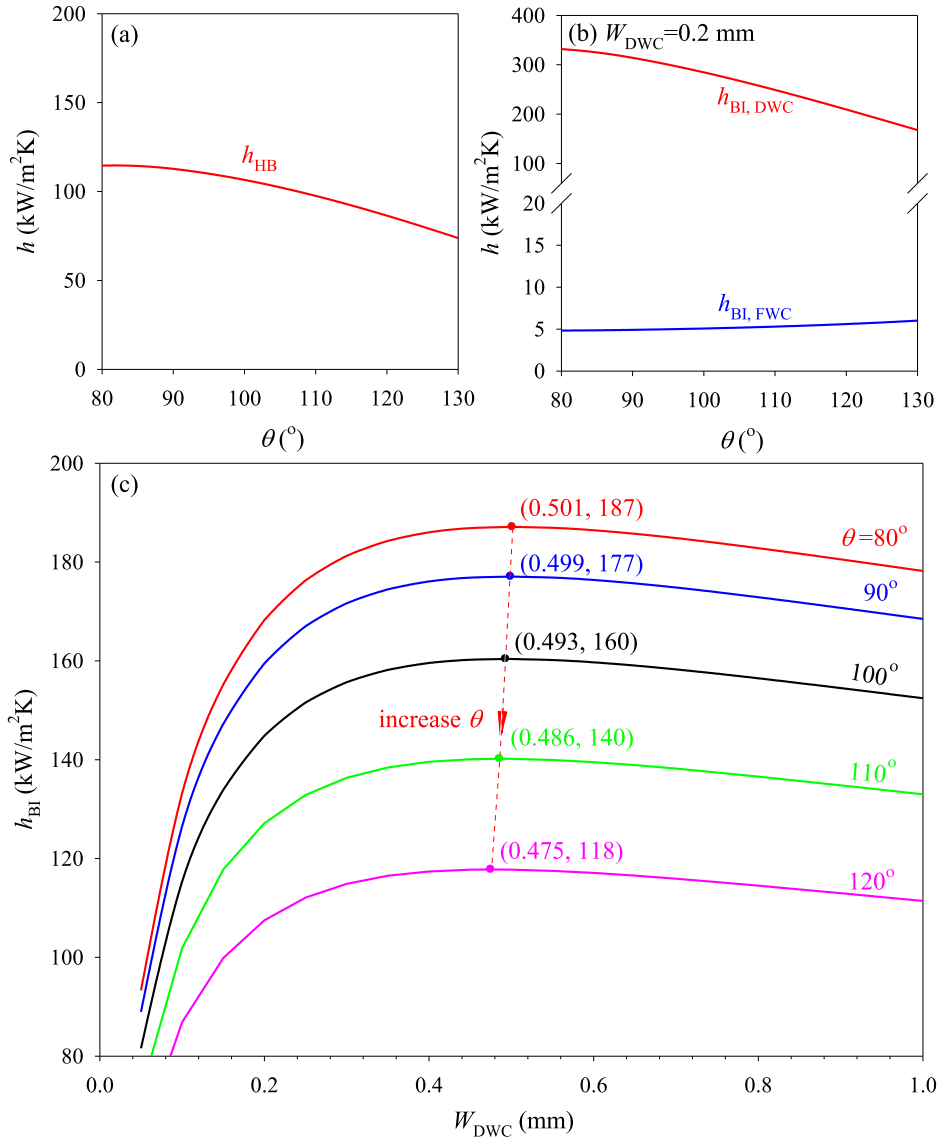
Fig. 11. Effect of equilibrium contact angle on heat transfer coefficients and optimal width of hydrophobic stripe ( T_{sat} = 60^\circ\text{C} , \Delta T = 5^\circ\text{C} , \theta_a = 120^\circ , \theta_r = 105^\circ , \delta_p = 1 nm, W_{FWC} = 0.2 mm).
